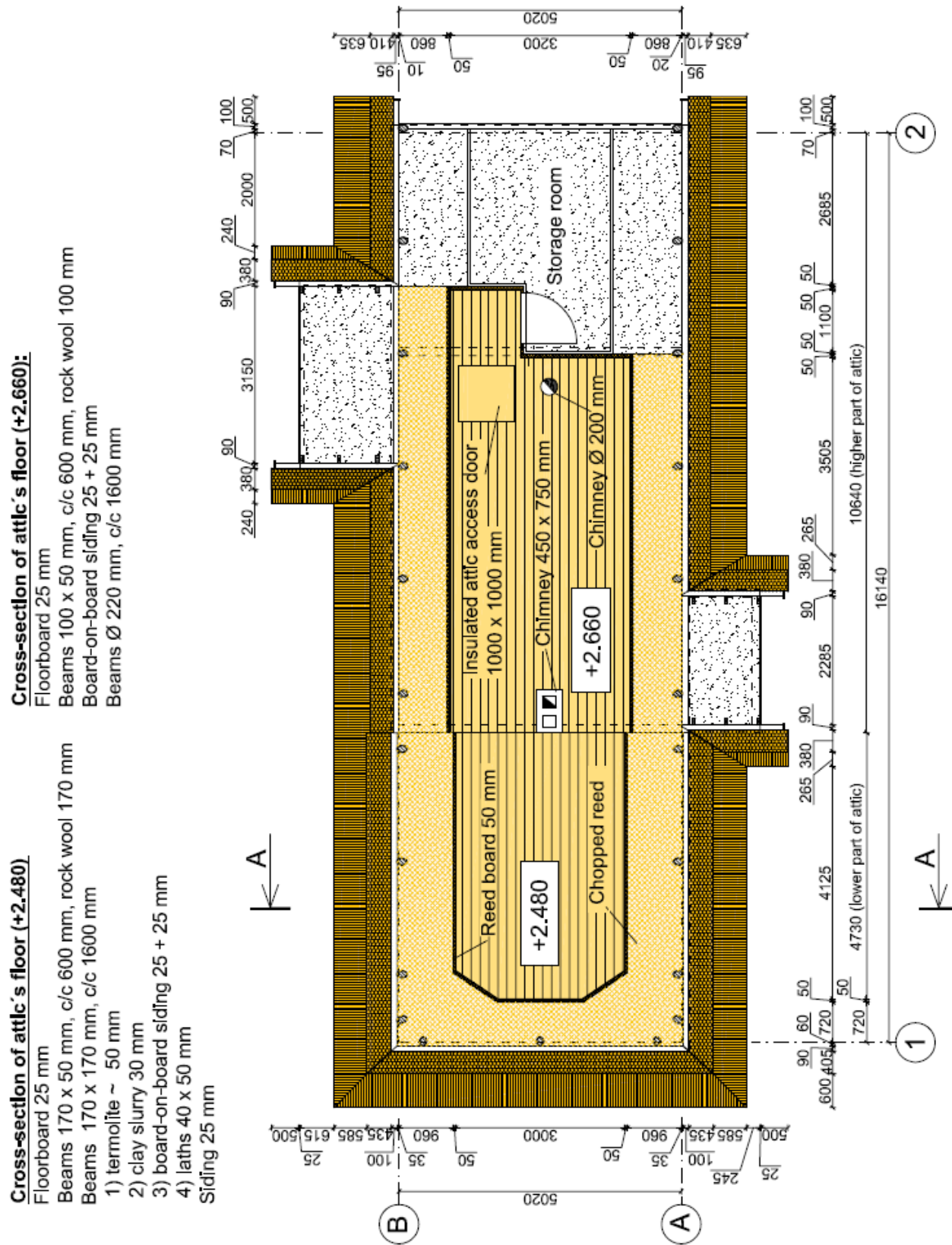
Figure 3.40 Plan of the attic floor of the farm on Hiiumaa (Lilleste 2013 b)
