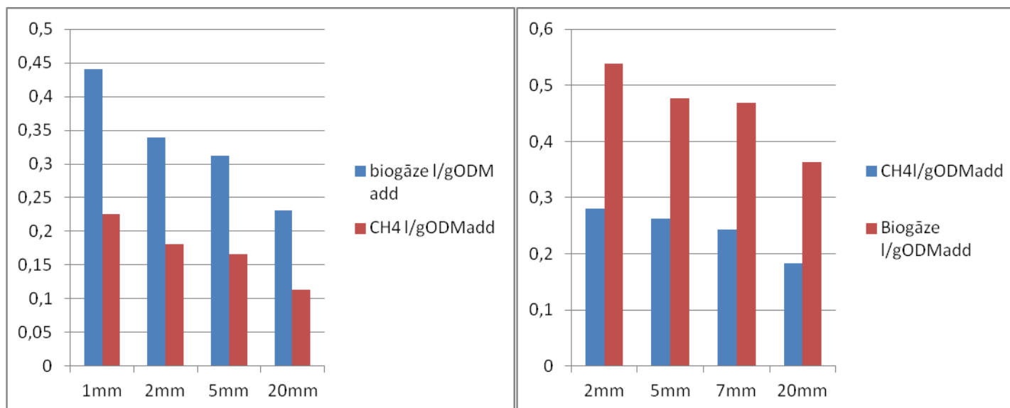
Figure 6.1 Average biogas and methane output, from winter reed, different cut sizes
