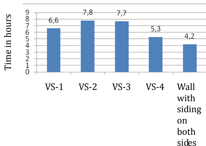
Figure 3.24 Comparison of construction times of reed insulated walls and lightweight wall
