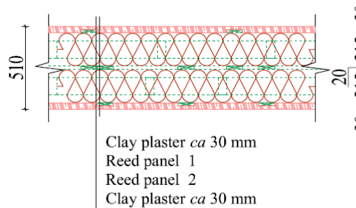
Figure 3.20 Different wall structures of test house
